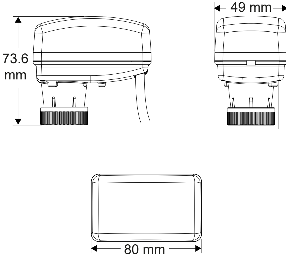
Figure 20: Actuator dimensions
